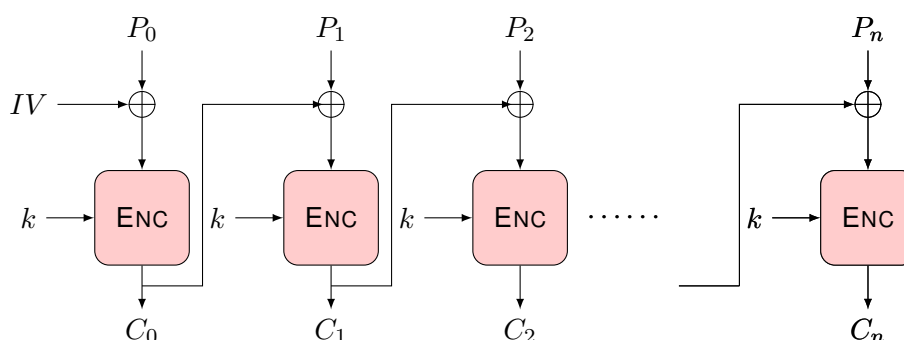
Figure 2: CBC Mode Encryption (All Figures are produced using TikZ for Cryptographers https://www.iacr.org/authors/tikz/ ).
